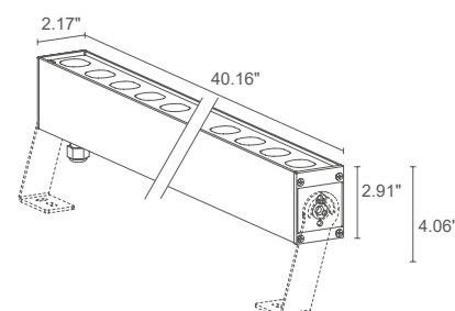
Fixture Dimensions
