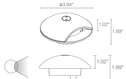
Fixture Dimensions
