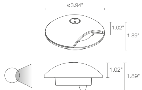
Fixture Dimensions
