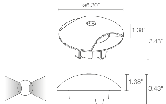
Fixture Dimensions
