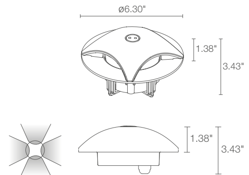
Fixture Dimensions
