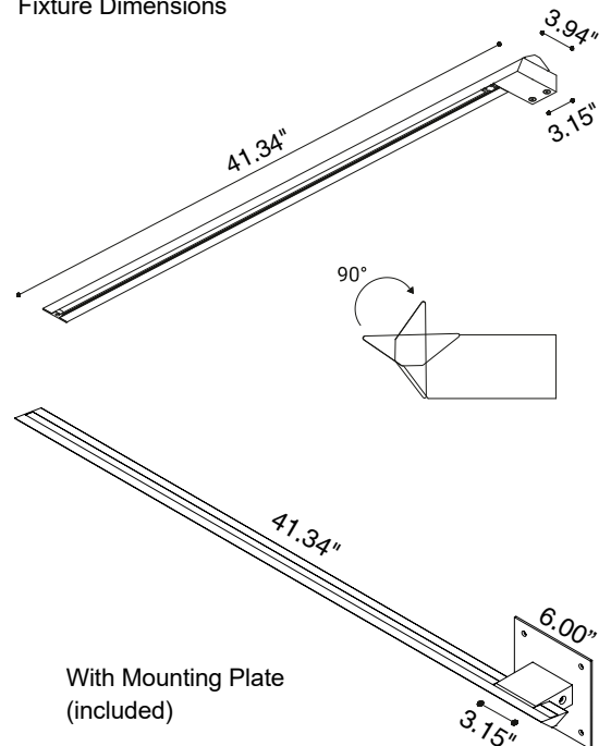
Fixture Dimensions
