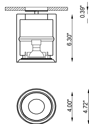
Fixture Dimensions
