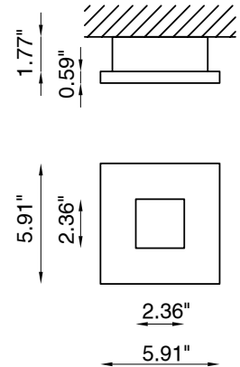
Fixture Dimensions
