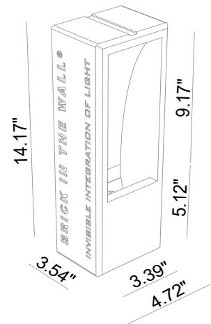
Wall Cut-Out: 4.88" l x 14.37" h Fixture Dimensions
