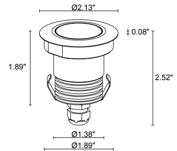
Fixture Dimensions
