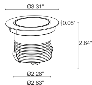
Fixture Dimensions
