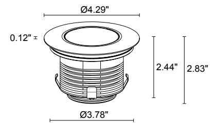
Fixture Dimensions
