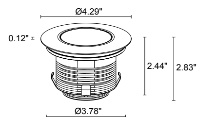
Fixture Dimensions
