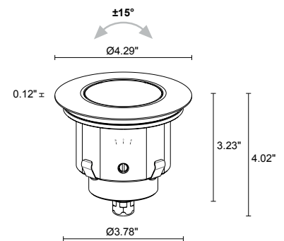
Fixture Dimensions
