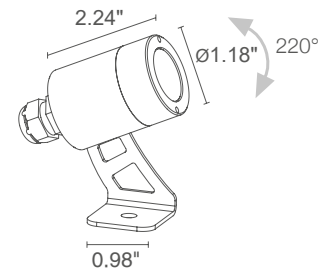
Fixture Dimensions
