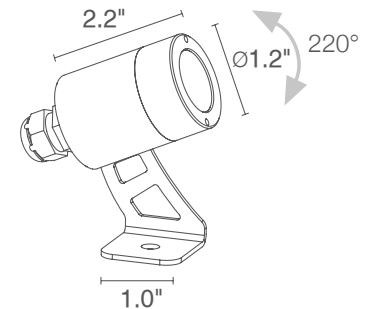
Fixture Dimensions
