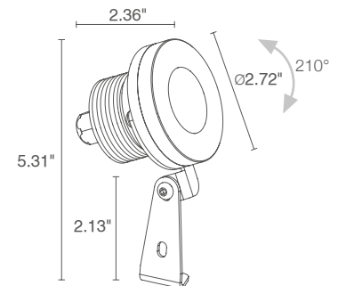
Fixture Dimensions
