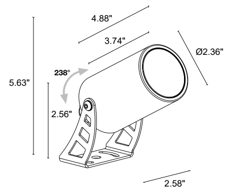
Fixture Dimensions
