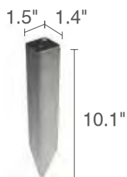
WP100 Ground Spike (10.1")
