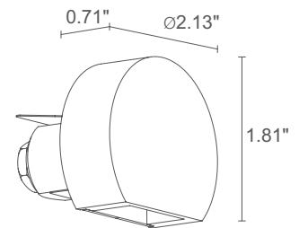
Wall Cut-Out: Ø1.18" Fixture Dimensions 2.13" l x .71" w x 1.81" h
