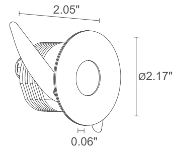
Wall Cut-Out: Ø1.77" Fixture Dimensions Ø2.17" x 2.05" I
