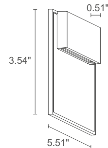
Fixture Dimensions 5.51" l x 0.51" w x 3.54" h
