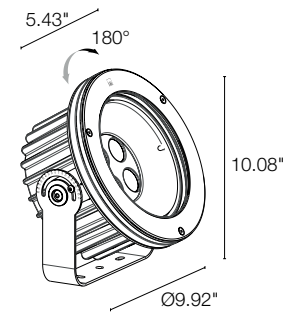
Fixture Dimensions
