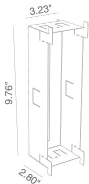
744 01 000 Outer Casing Housing: perforated aluminum
