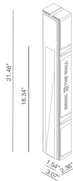
Ceiling Cut-Out: 3.27" × 21.65" Fixture Dimensions
