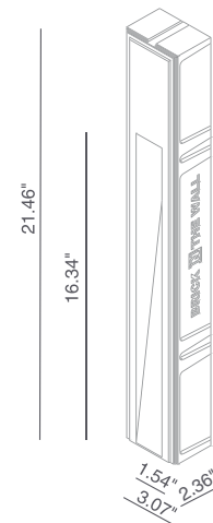
Ceiling Cut-Out: 3.27" × 21.65" Fixture Dimensions
