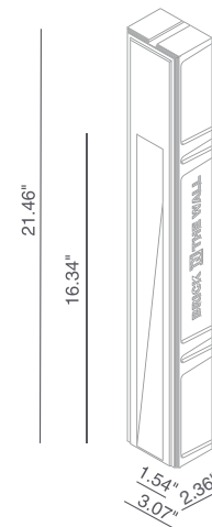
Ceiling Cut-Out: 3.27" × 21.65" Fixture Dimensions
