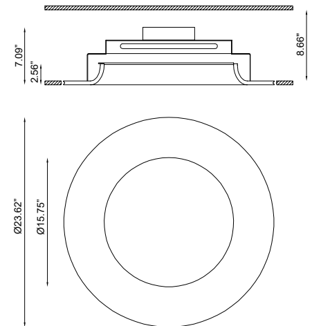
Fixture Dimensions
