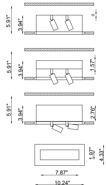
Fixture Dimensions
