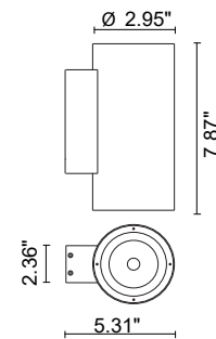
Fixture Dimensions
