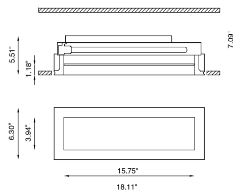
Fixture Dimensions
