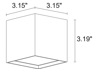
Fixture Dimensions
