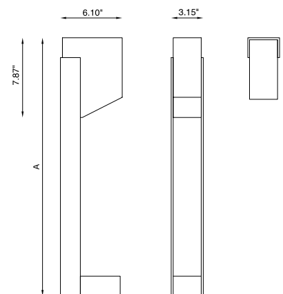
Fixture Dimensions
