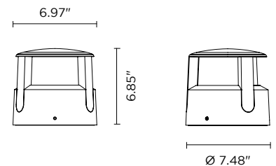
Fixture Dimensions
