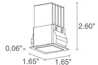
Cut-Out Dimensions: 1.46" x 1.46" Fixture Dimensions
