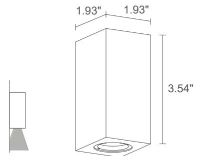
Fixture Dimensions
