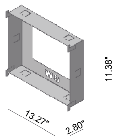
720 01 000 Outer Casing
