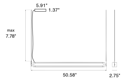
Fixture Dimensions
