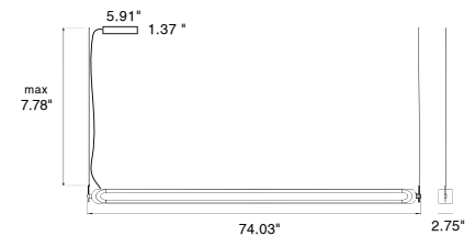
Fixture Dimensions
