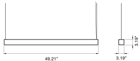
Fixture Dimensions
