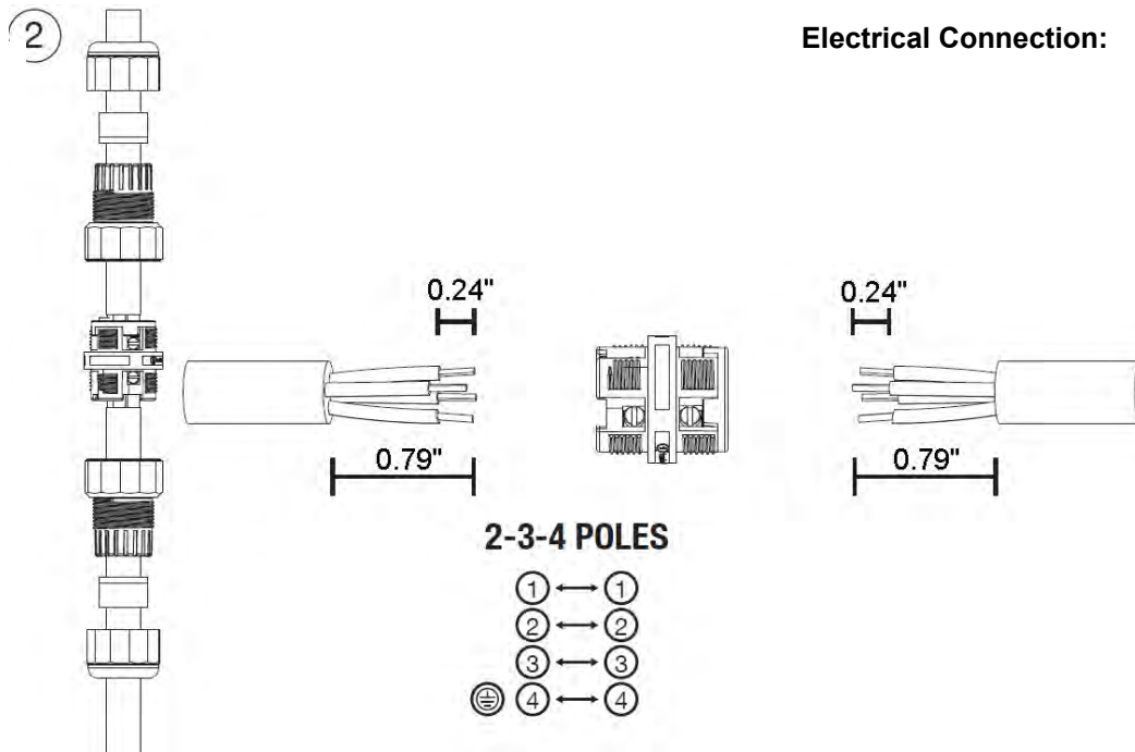
3/4 way connector (optional)
