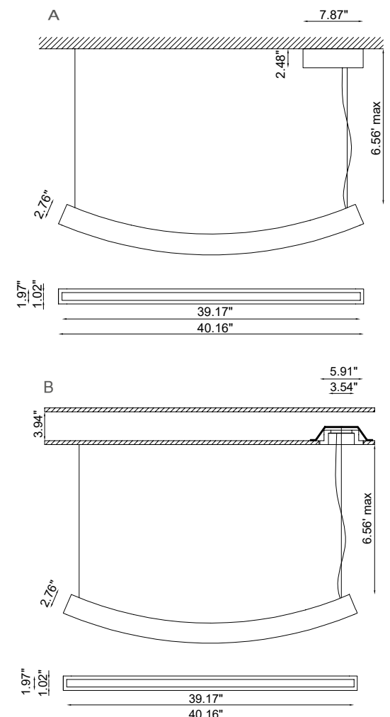
Fixture Dimensions
