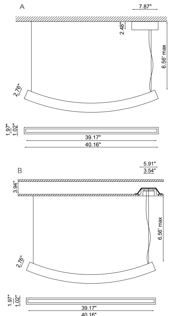
Fixture Dimensions
