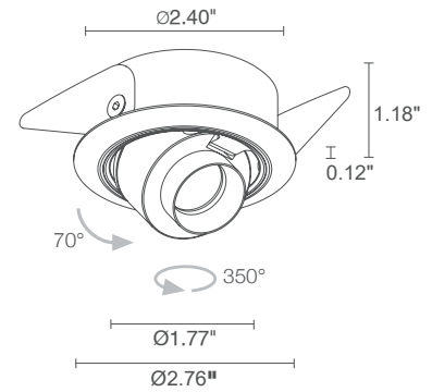
Ceiling Cut-Out: Ø2.56" Fixture Dimensions Ø2.40" x 1.18" h x Ø2.76" outer rim
