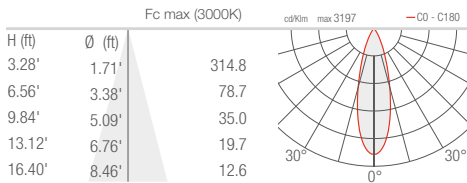
M - 29° CRI 90 - flat, square cover
