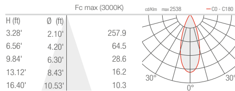
L - 36° CRI 90 - shallow, square cover
