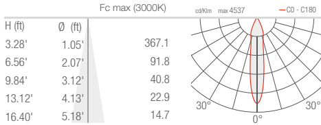
S - 18° CRI 90 - flat, square cover
