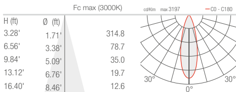
M - 29° CRI 90 - shallow, square cover
