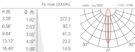
S - 18° CRI 90 - deep, square cover
