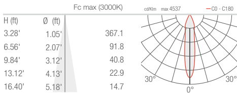
S - 18° CRI 90 - shallow, square cover
