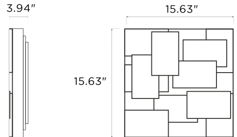
Fixture Dimensions
