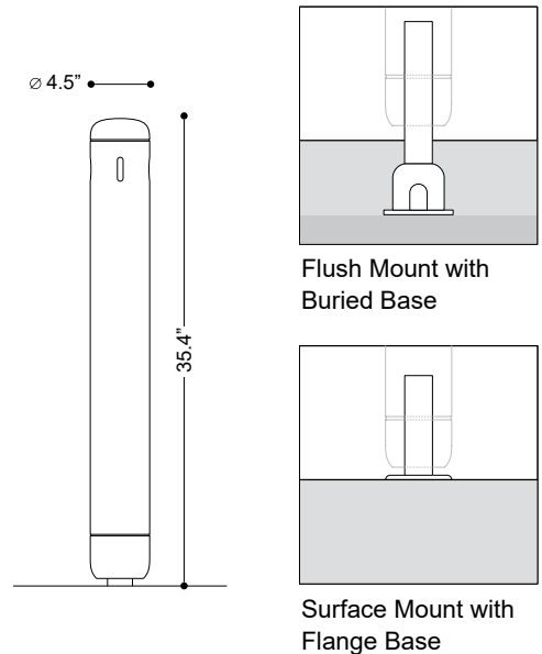
Fixture Dimensions Ø4.5" x 35.4" h
