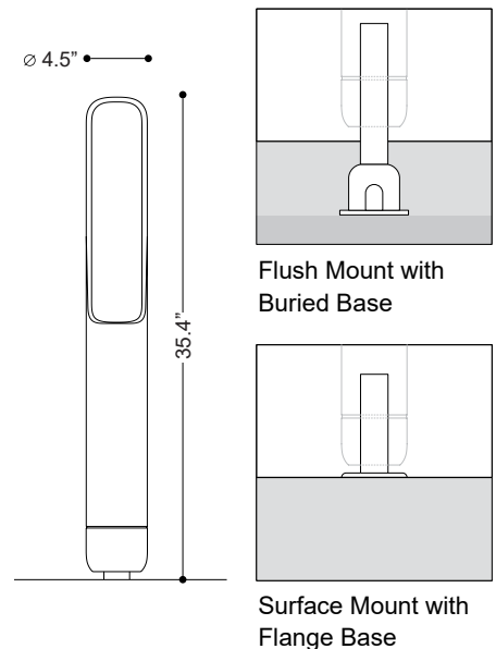
Fixture Dimensions Ø4.5" x 35.4" h
