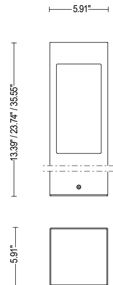
Fixture Dimensions
