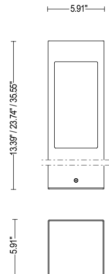
Fixture Dimensions
